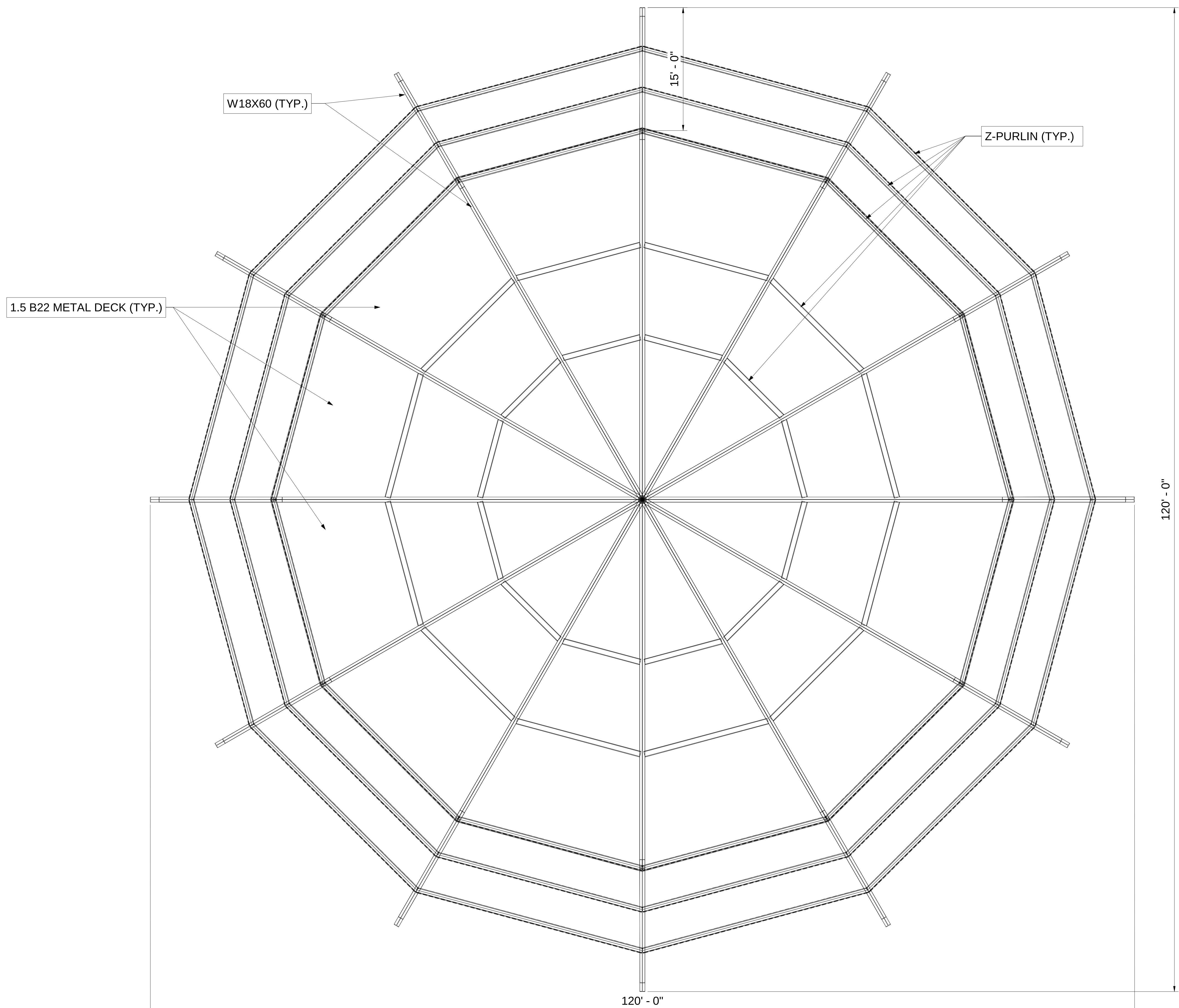
1 FRAMING PLAN 3/16" = 1'-0"
