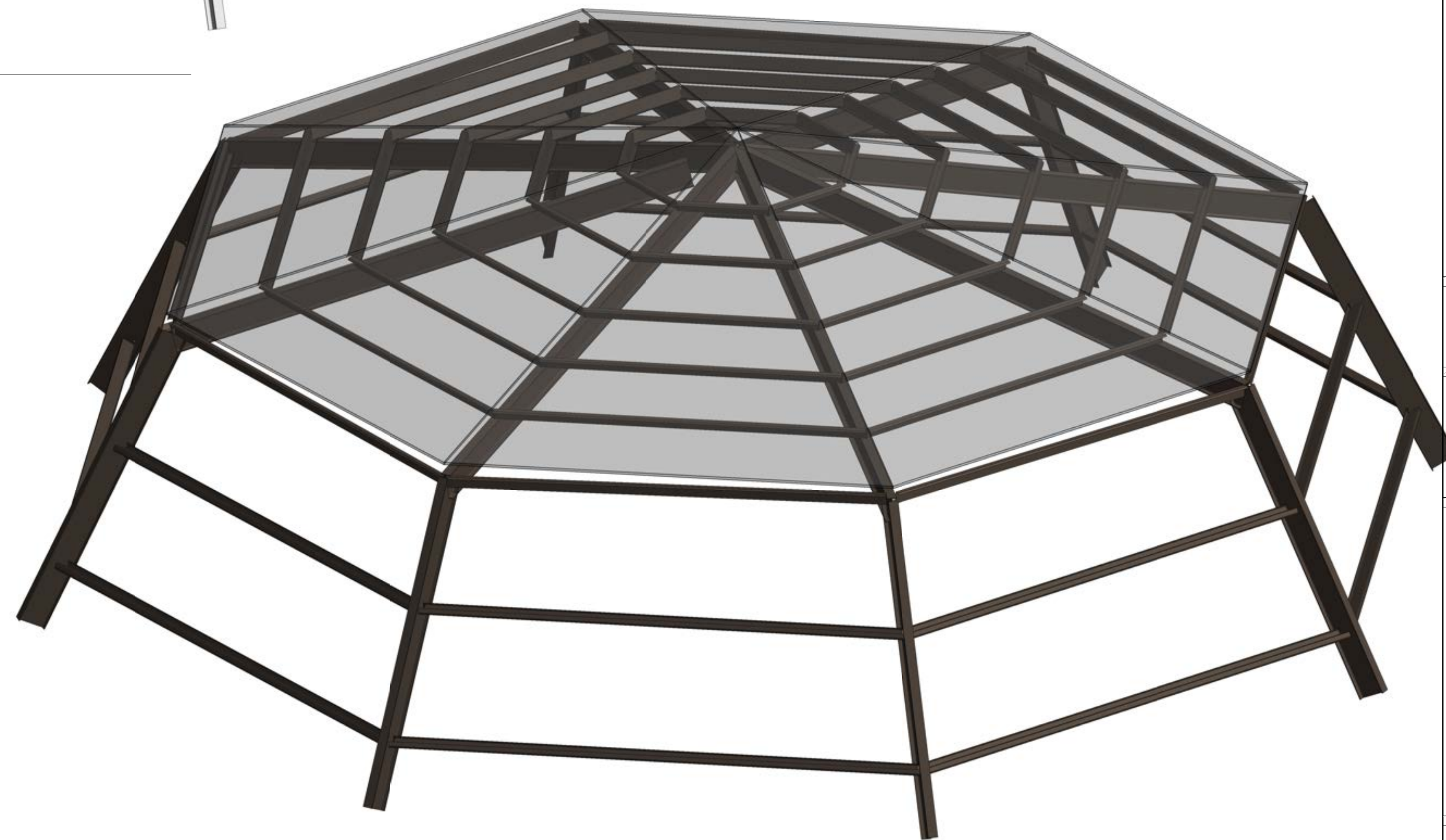
2 3D VIEW
