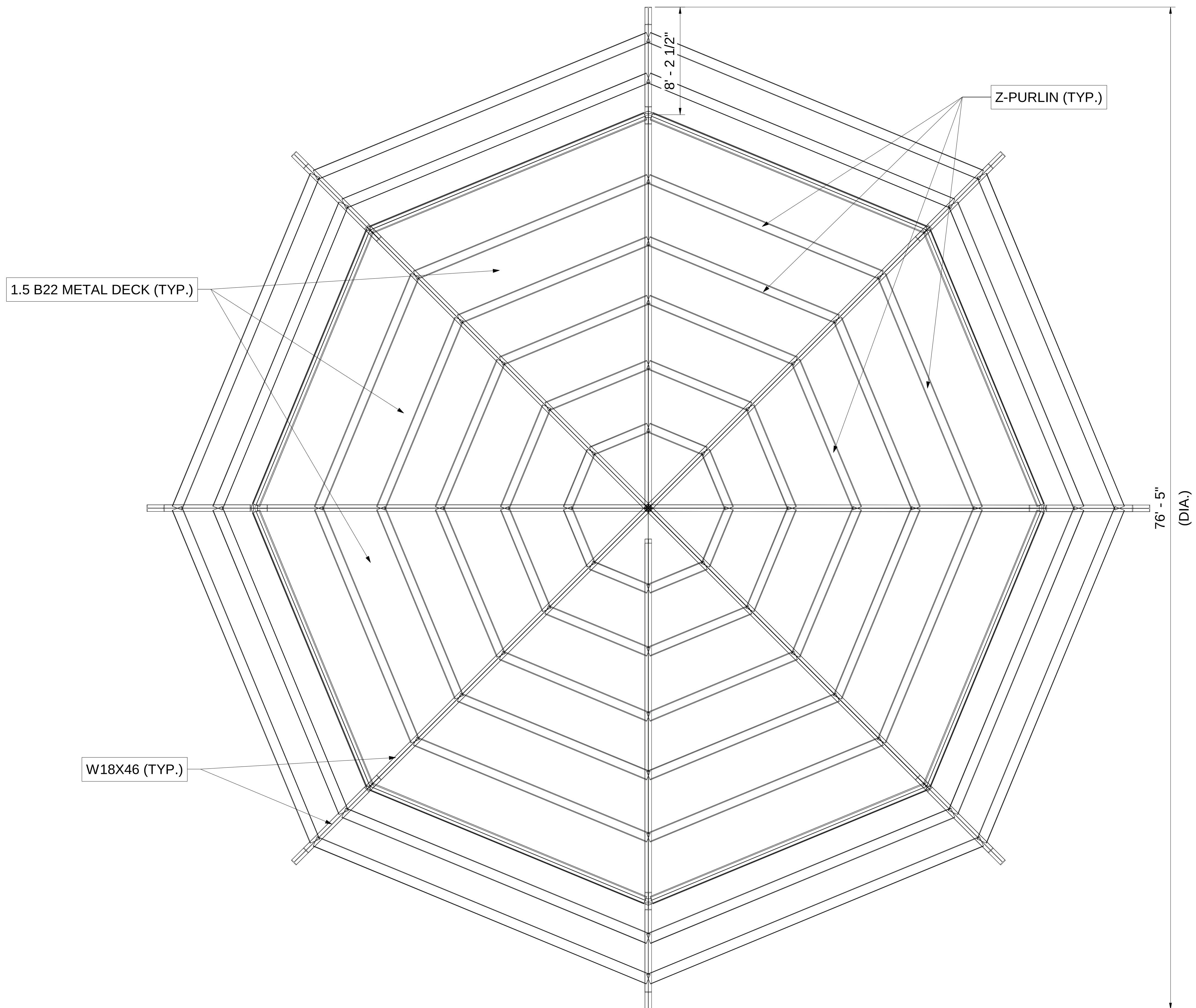
1 FRAMING PLAN 1/4" = 1'-0"
