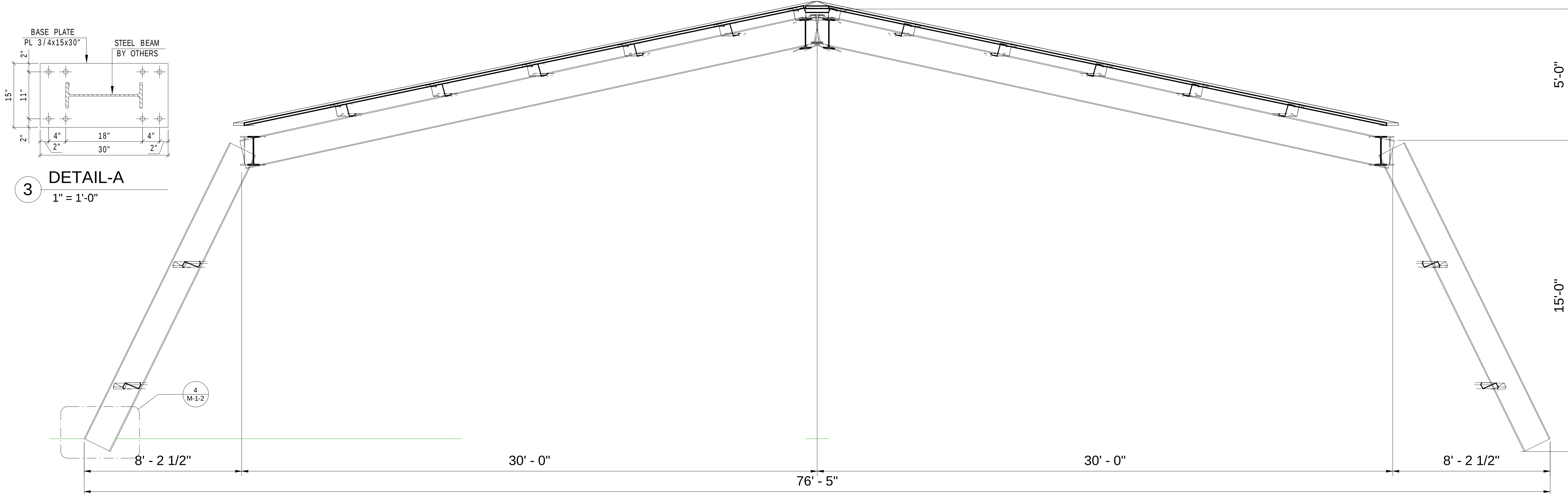
2 ELEVATION 3/8" = 1'-0"
