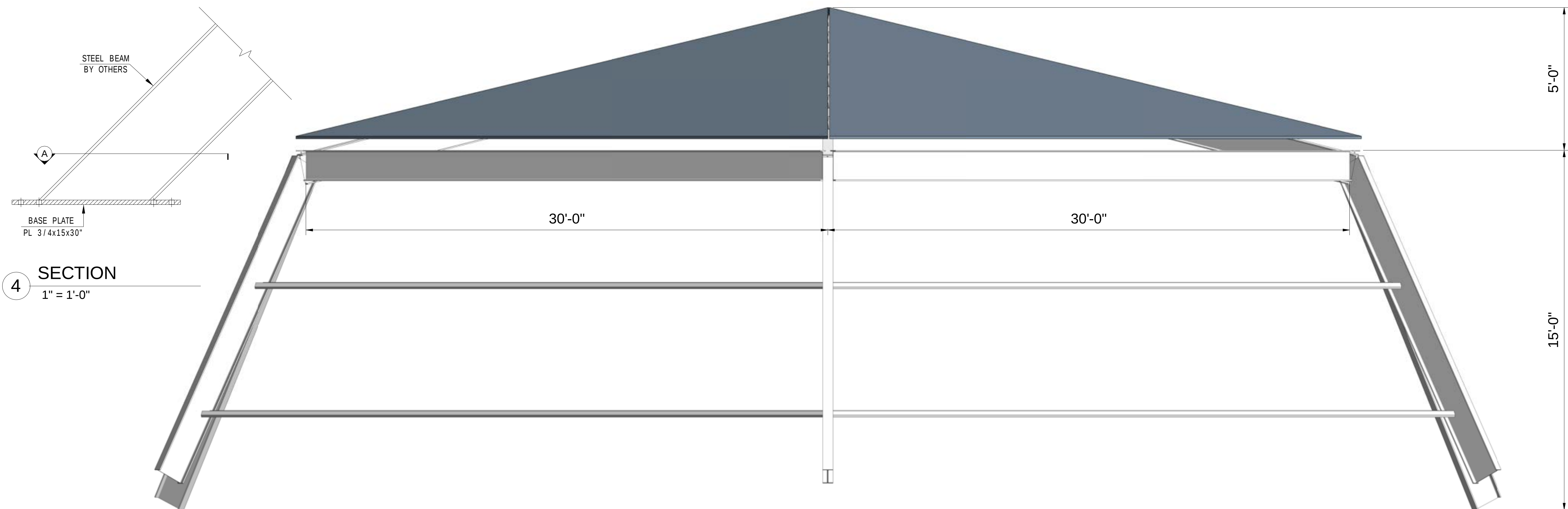
1 ELEVATION 3/8" = 1'-0"
