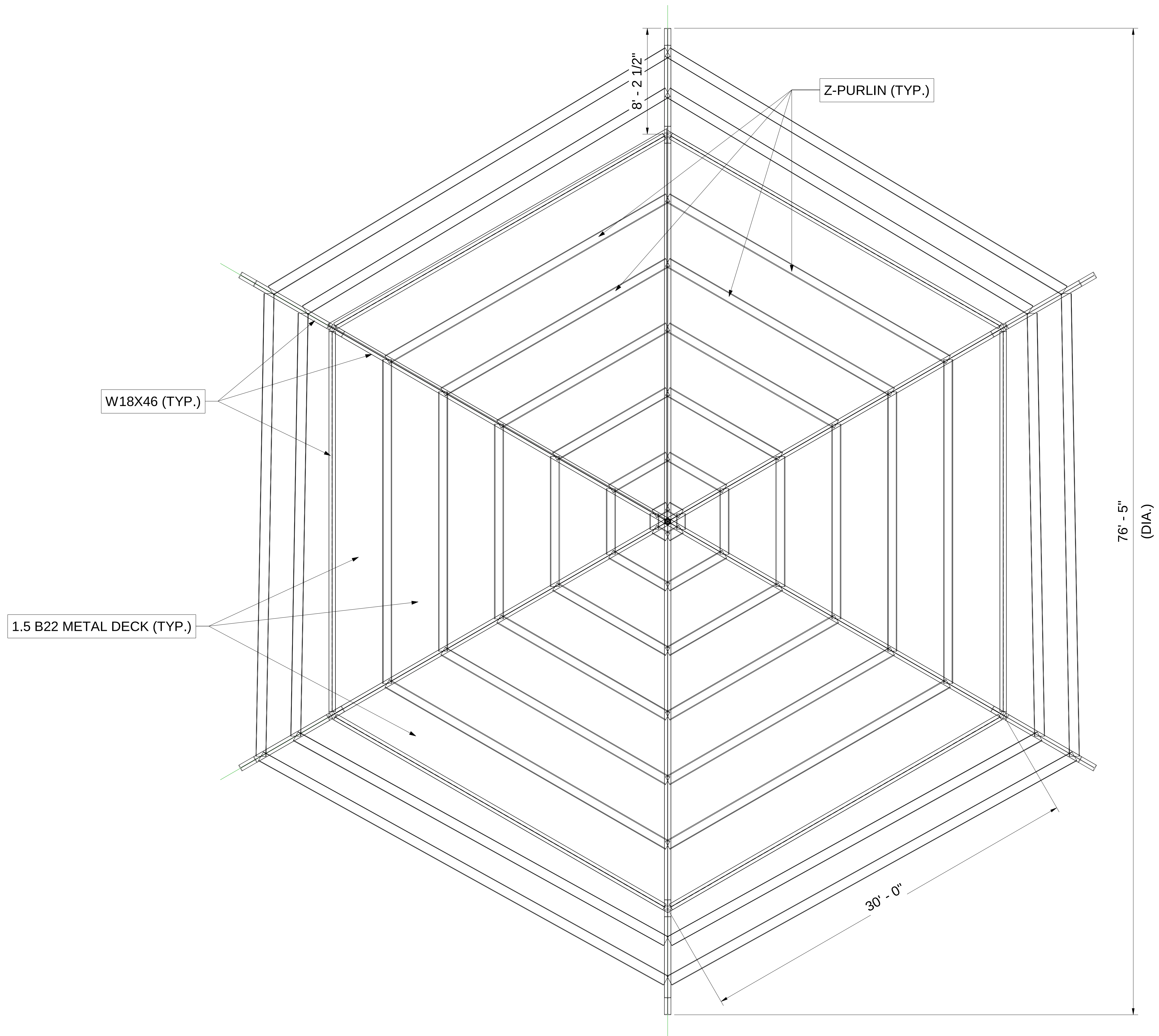
1 FRAMING LAYOUT PLAN 1/4" = 1'-0"
