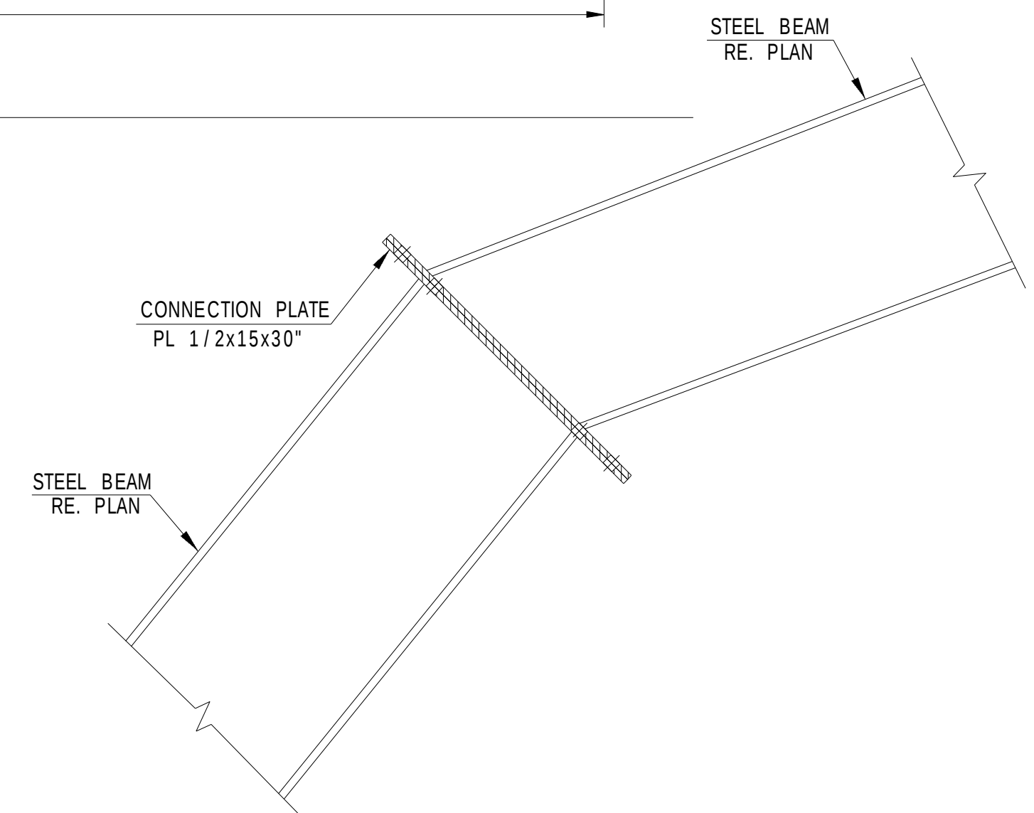
6 SECTION 1" = 1'-0"
