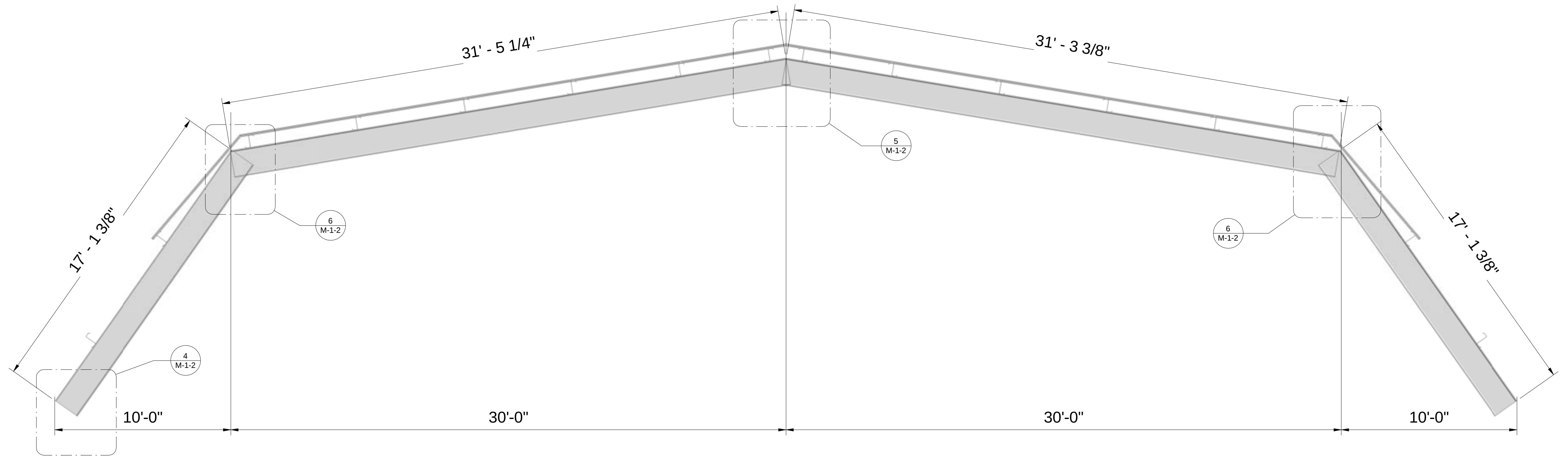
1 FRONT & REAR VIEW 1 : 40
