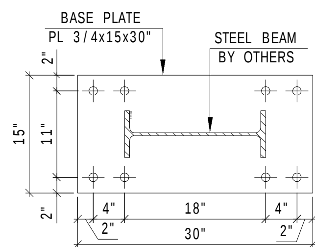
3 DETAIL-A 1" = 1'-0"
