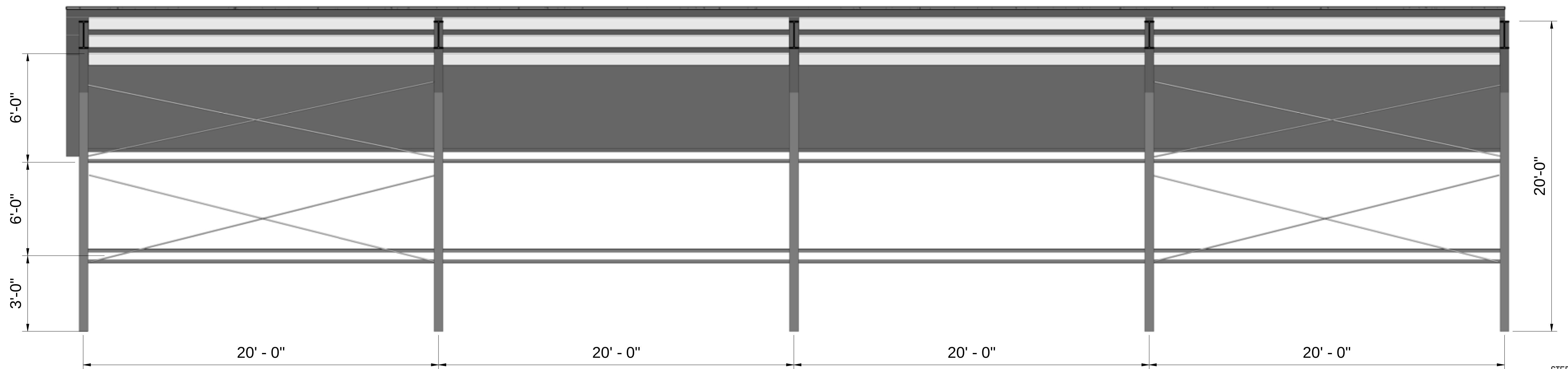
2 SIDE VIEW 1 : 40
