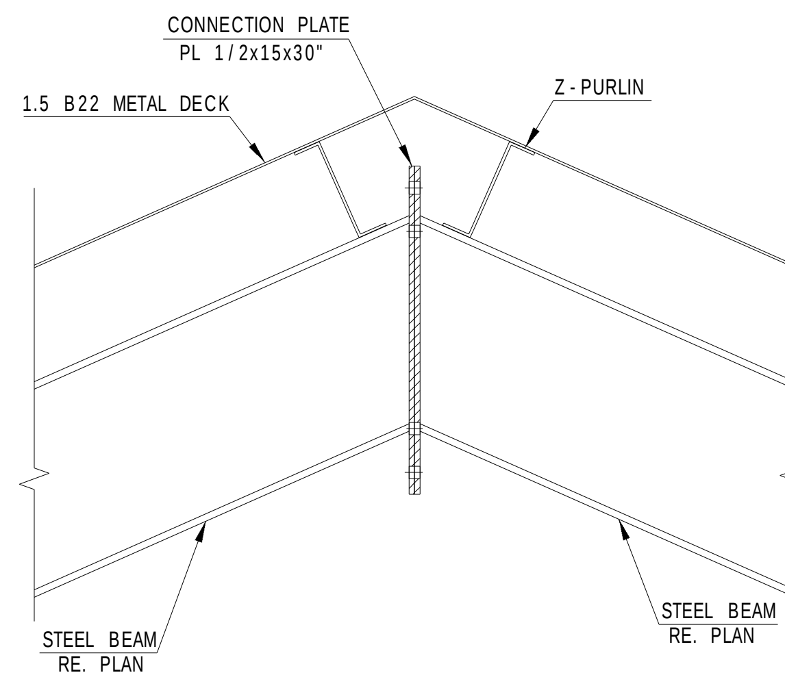
5 SECTION 1" = 1'-0"
