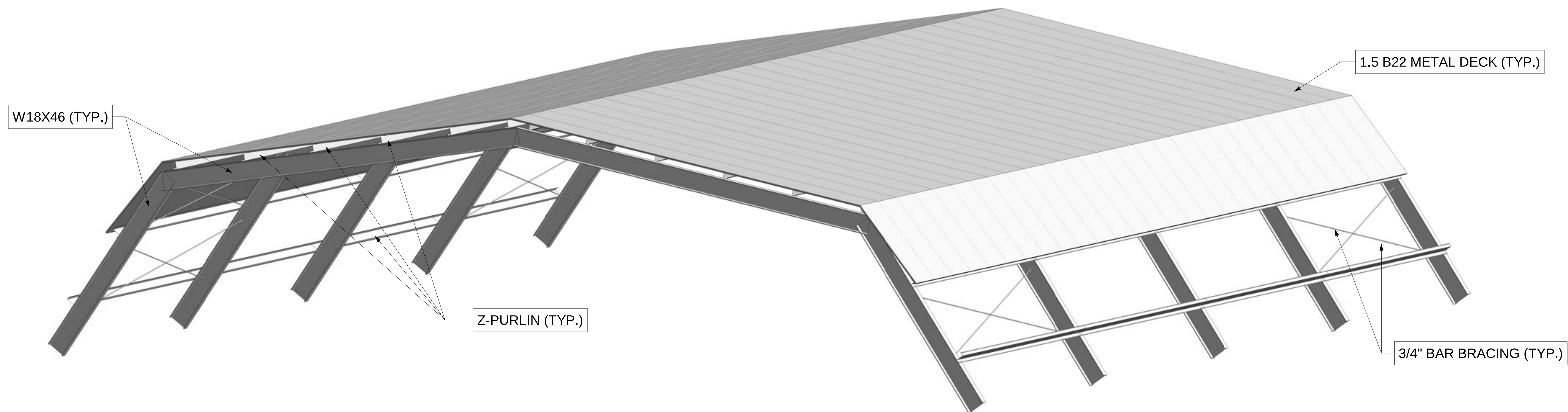
1 3D VIEW
