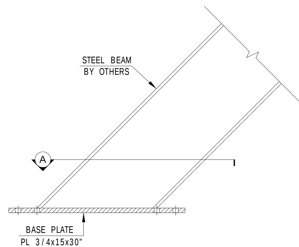
4 SECTION 1" = 1'-0"
